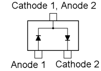
DA221 (K) (D2001, 2002, 2005, 2009, 2012, 2013, 2036)
